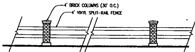
4' RAIL FENCE DETAIL
