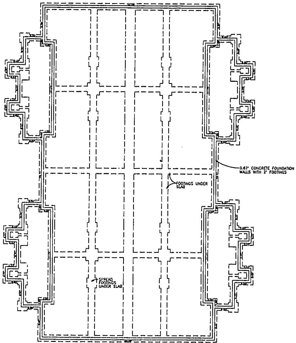
FOOTINGS AND FOUNDATION (BUILDING 6163)
