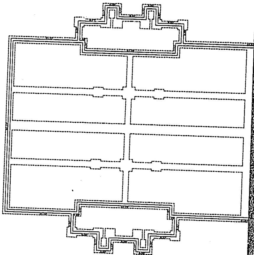
FOOTINGS AND FOUNDATION
