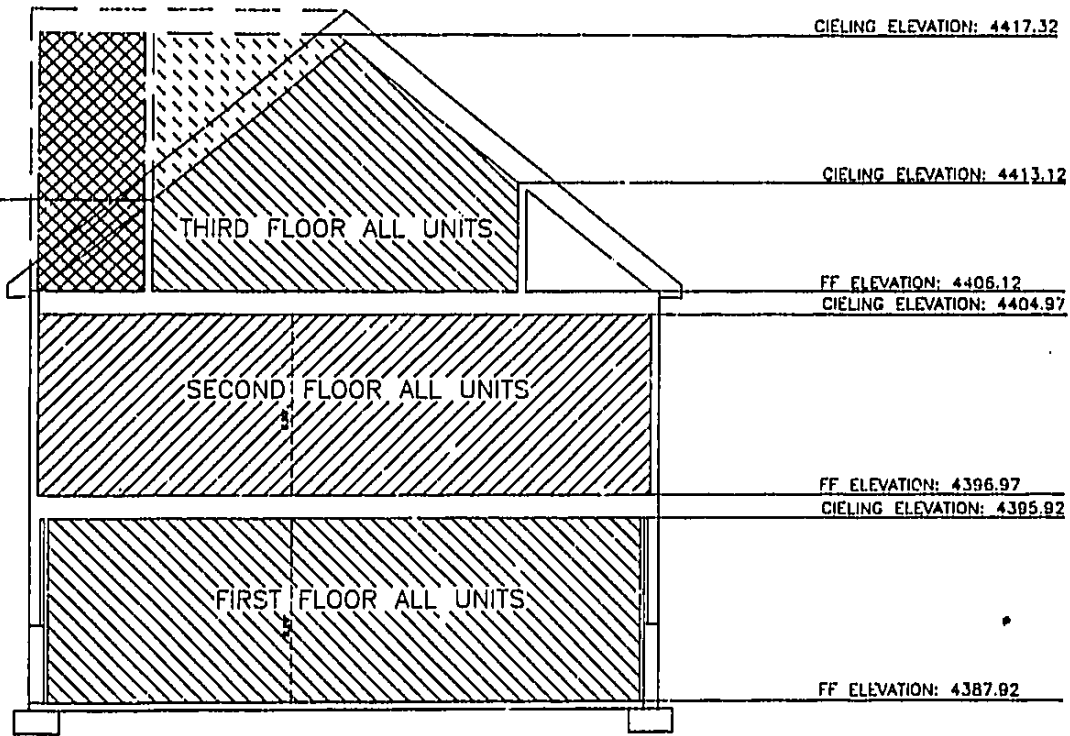
ELEVATION PLAN (BUILDING 6165)
