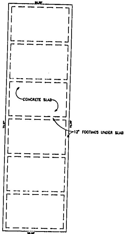
FOOTING AND FOUNDATION PLAN
