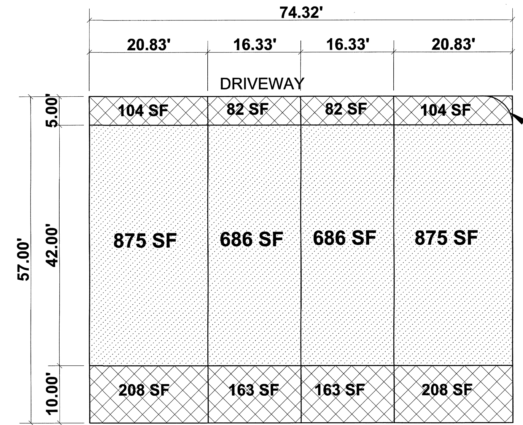
FRONT MAIN FLOOR PLAN 4-PLEX (LOTS 147-150, 155-158)
