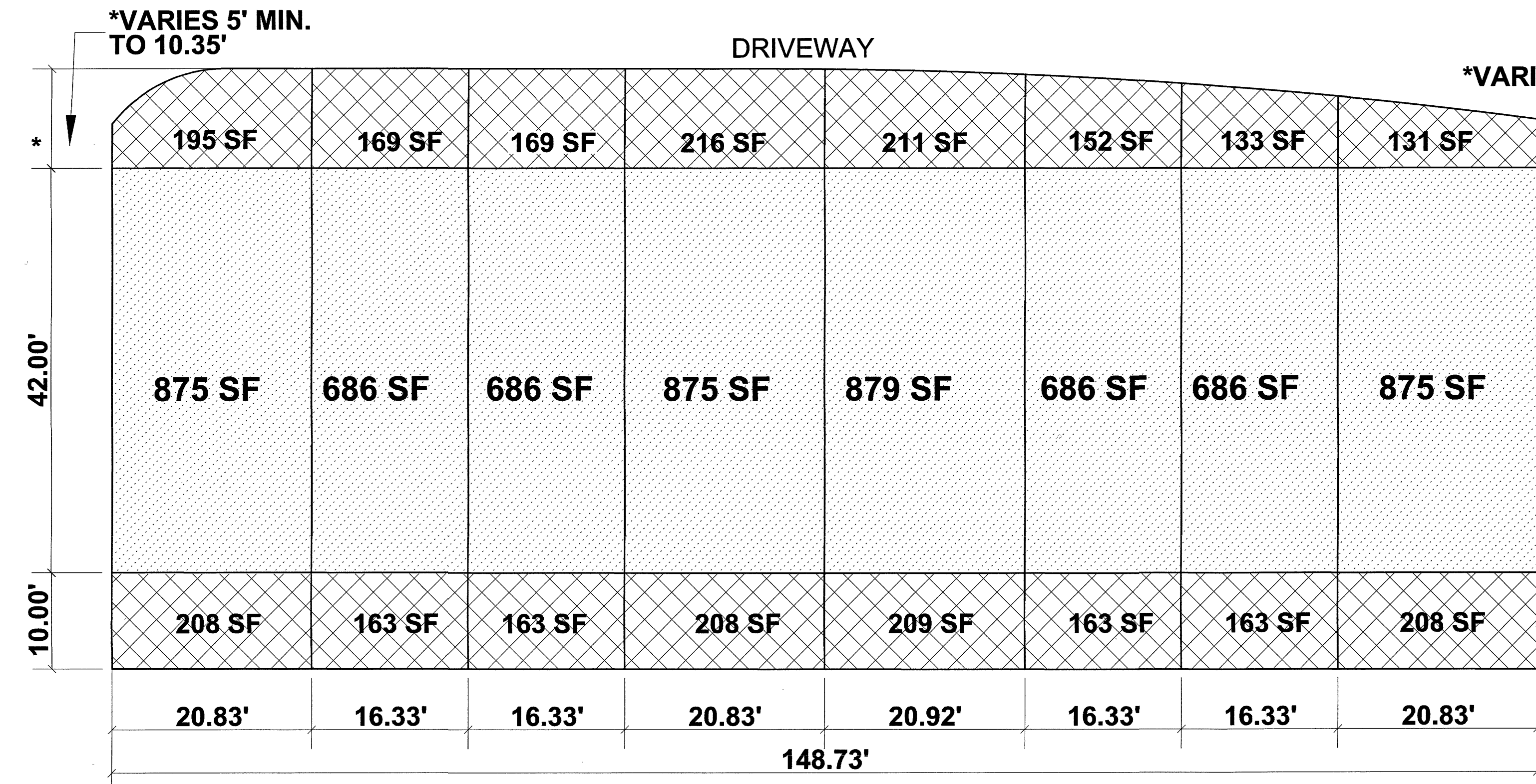
MAIN FLOOR PLAN 8-PLEX (LOTS 171-178)
