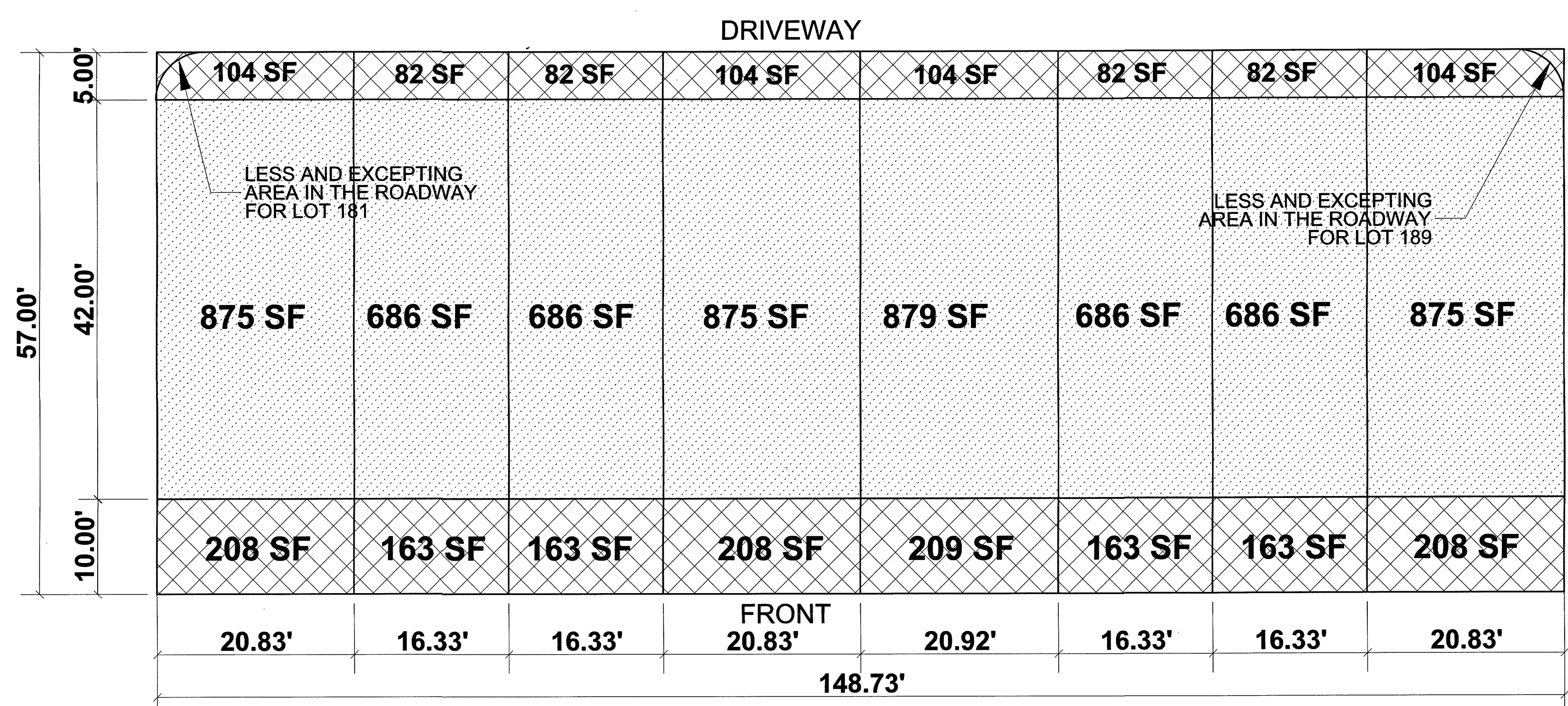
MAIN FLOOR PLAN 8-PLEX (LOTS 159-166, 181-196)
