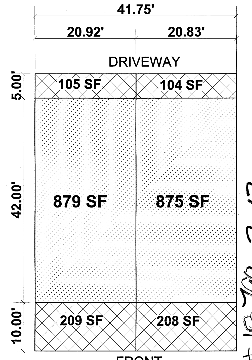
FRONT MAIN FLOOR PLAN DUPLEX (LOTS 151-154, 179-180)
