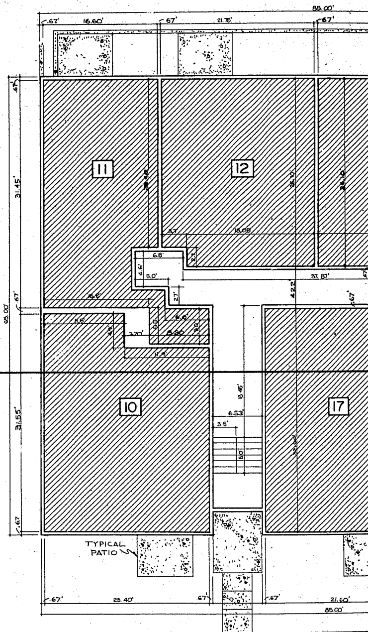
FIRST FLOOR PLAN SCALE: 1" = 6'
