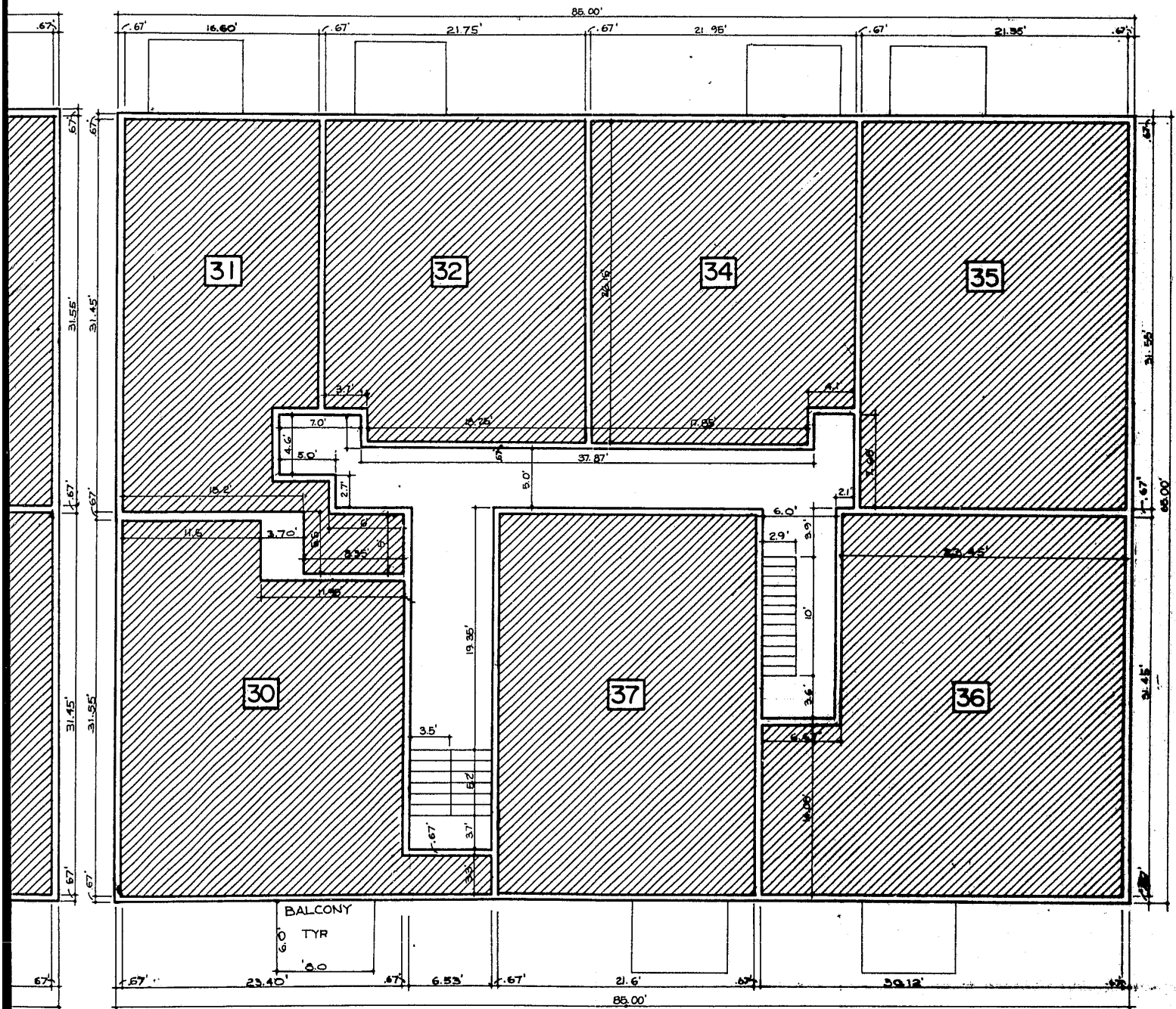
THIRD FLOOR PLAN SCALE: 1" = 6'
