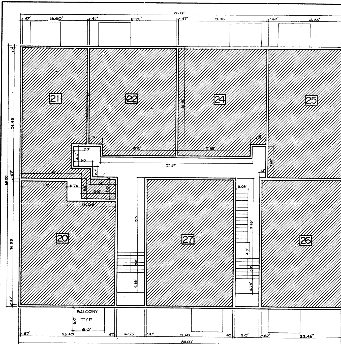
SECOND FLOOR PLAN SCALE: 1" = 6'
