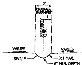
DRAINAGE SWALE DETAIL N.T.S.
