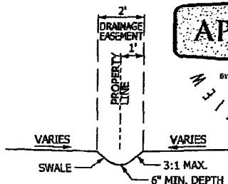
DRAINAGE SWALE DETAIL N.T.S.
