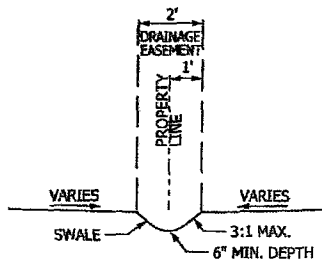
DRAINAGE SWALE DETAIL R.T.S.
