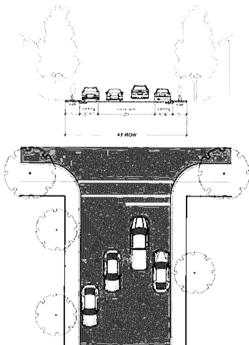
Figure 3.1 Typical Private Street
