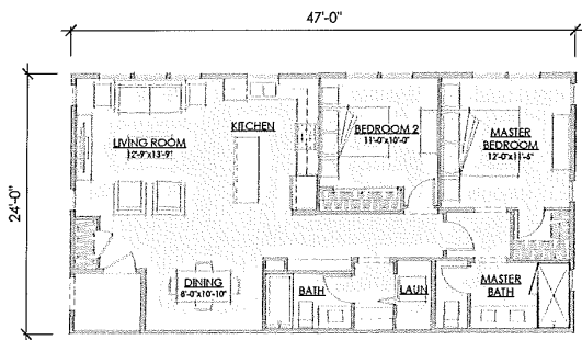
PLAN 4 2 BR, 2 BA: 1,092 SF 80 UNITS
