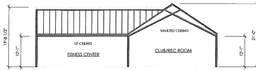
SECTION A
