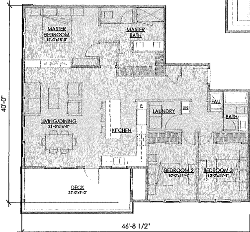
PLAN 3 3 BR, 2 BA: 1,443 SF 64 UNITS
