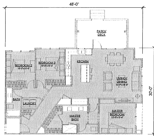
PLAN 5 3 BR, 2 BA: 1,367 SF 120 UNITS
