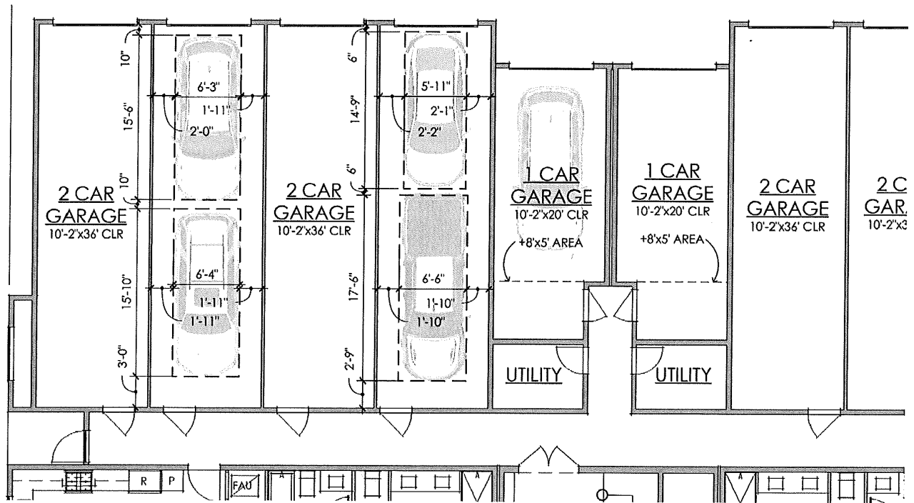
FIRST FLOOR: TANDEM GARAGE DETAIL
