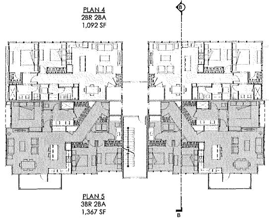
SECOND AND THIRD FLOORS
