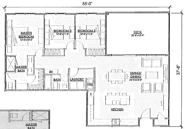
PLAN 2 3 BR, 2 BA: 1,426 SF 64 UNITS
