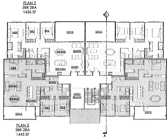
SECOND AND THIRD FLOORS
