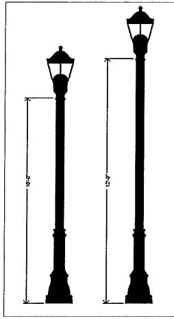
LIGHT FIXTURE
