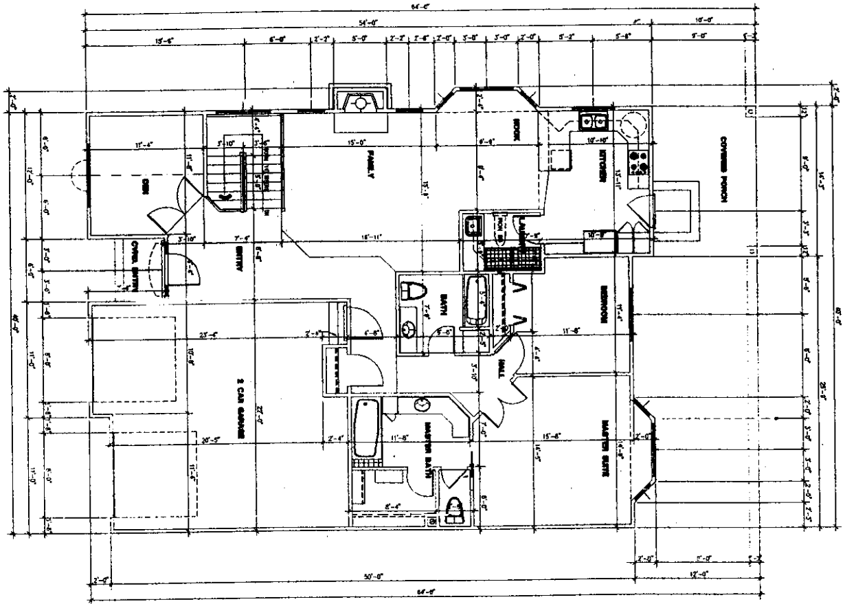
MAIN FLOOR PLAN SCALE: 1/4" = 1'-0" 1973 SQ FT
