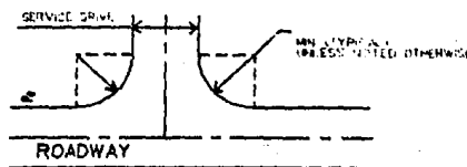
(B) CURB CUT DETAIL 1"=100'-0"
