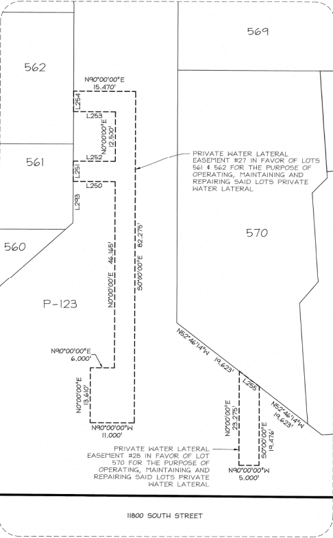
DETAIL "TT" SCALE: 1" = 10'
