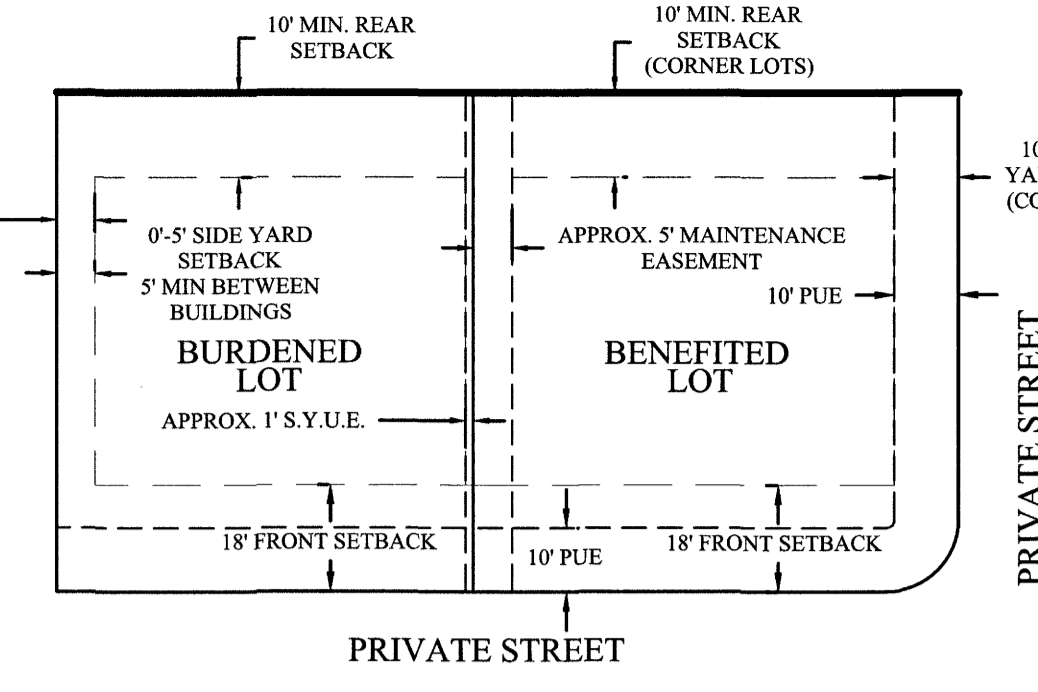
TYPICAL FRONT LOAD SINGLE FAMILY BUILDING SETBACKS LOTS 224-231
