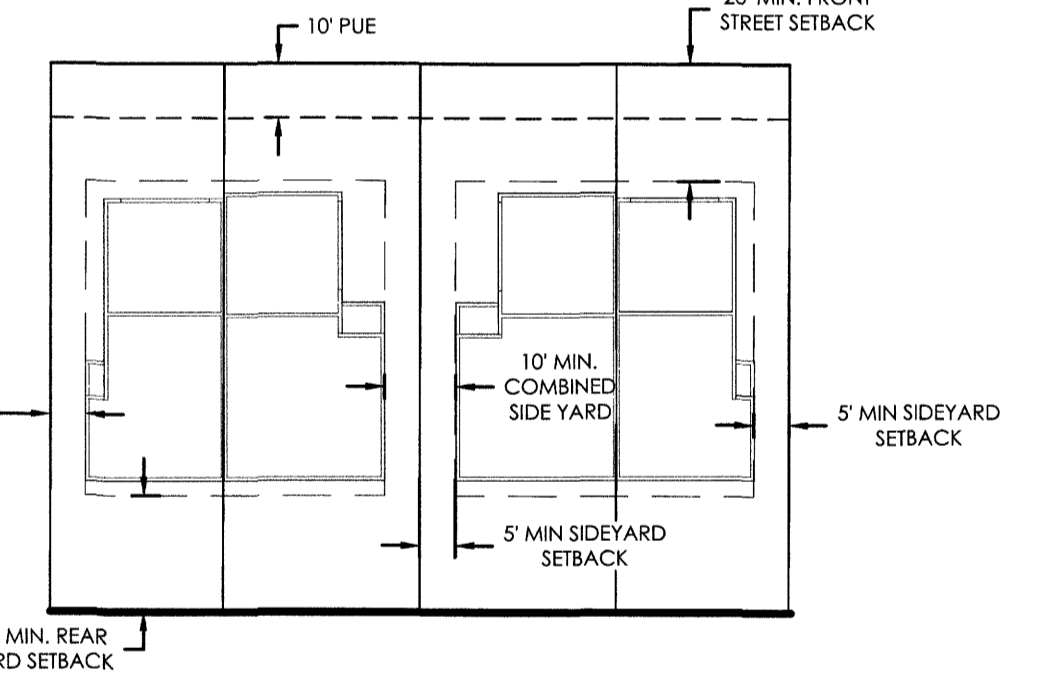
TYPICAL PAIRED HOME SETBACKS LOTS 201-216
