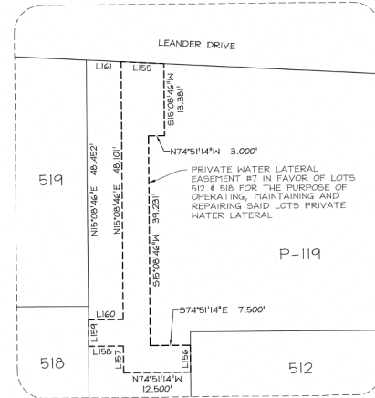
DETAIL "MM" SCALE: 1" = 10'
