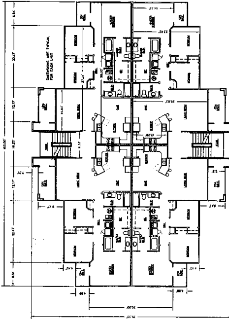
2ND LEVEL FLOOR PLAN BUILDINGS A-3 (UNITS 401-440) SEE SHEET 1 OF 2 FOR UNIT ASSIGNMENT TO BUILDING QUADRANT
